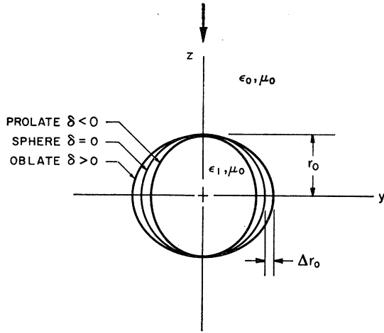
FIG. 2. The dielectric spheroid. The arrow indicates the direction of the incident wave.
