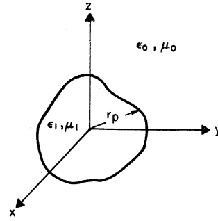
FIG. 1. The arbitrarily shaped dielectric body.
