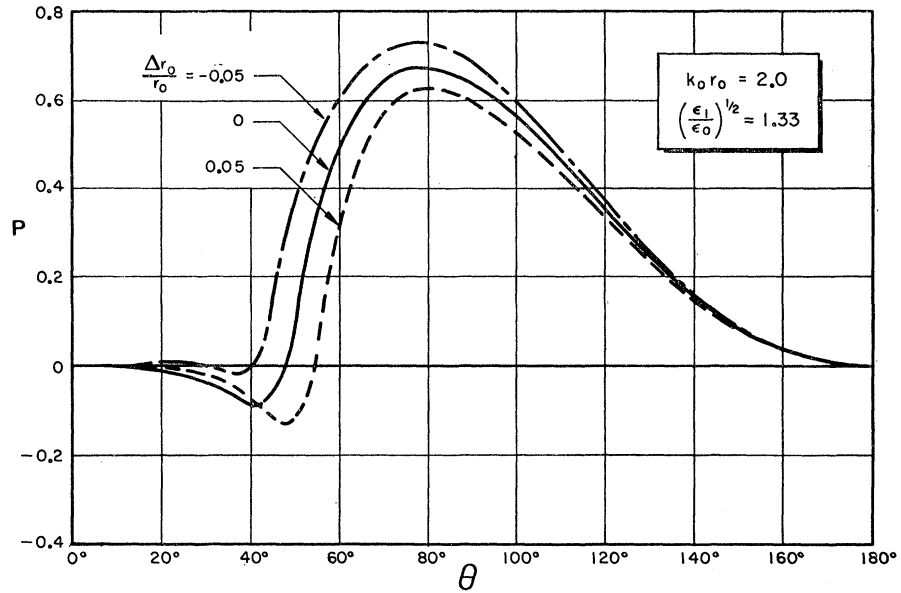
FIG. 4. The polarization of light scattered from dielectric spheroid for nose-on incidence.
