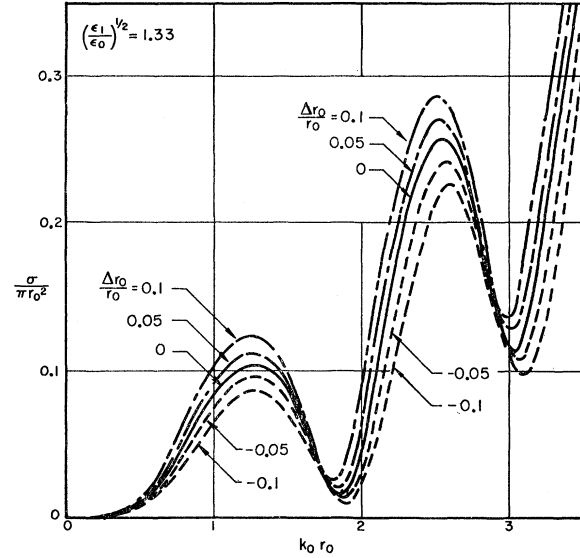
FIG. 3. The normalized backscattering cross sections for nose-on incidence.
